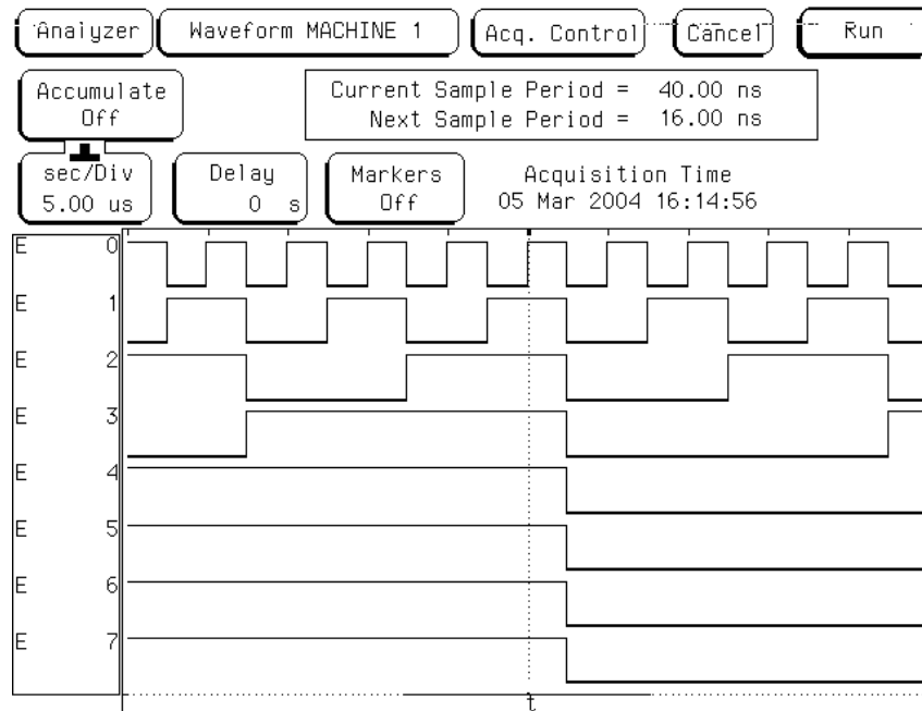
Figure 6: Commstime output from logic analyzer.
